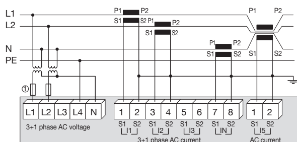
Connection with VT : 2 phases + neutral, 3 wires, 3 CT (2.3.3)
