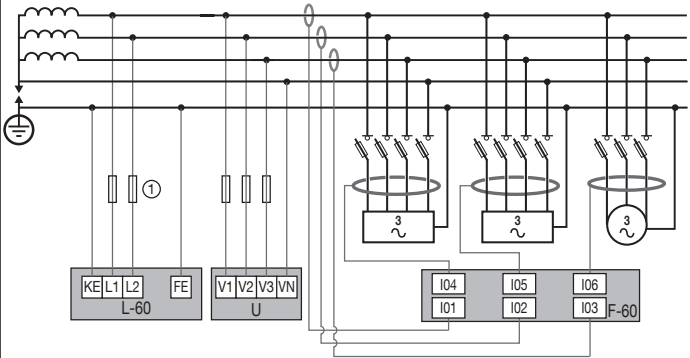
3AC+N / IMD + IFL + upstream load current monitoring
