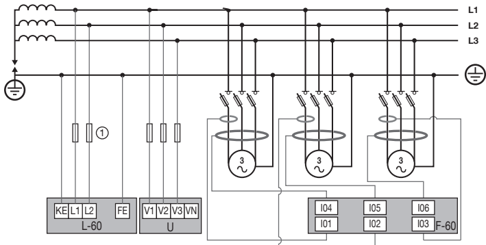
3AC / IMD + IFL + load current monitoring
